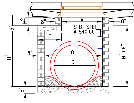
END ELEVATION SECTION Y-Y
