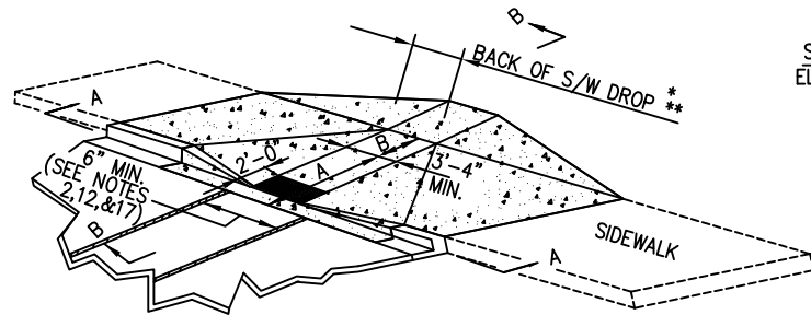
ISOMETRIC VIEW
