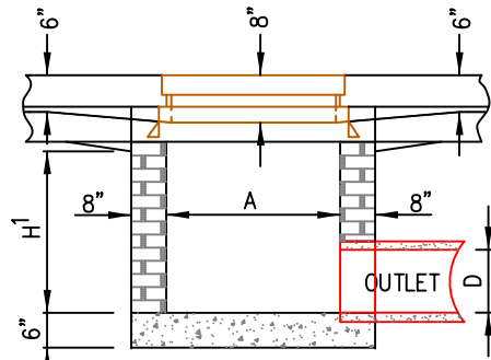
SECTION Y-Y
