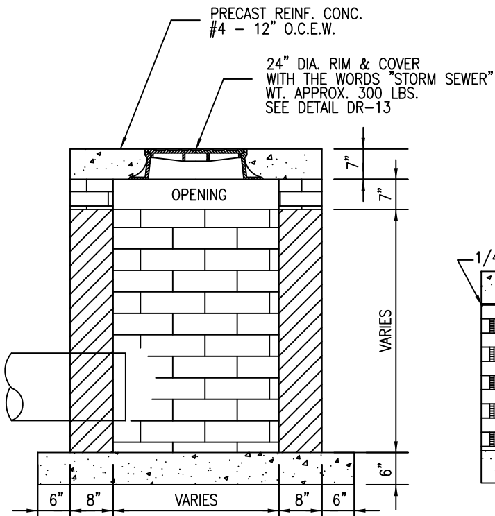
SECTION - XX
