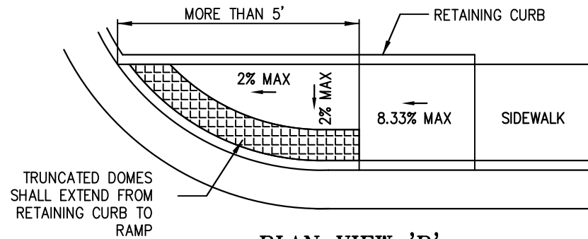
PLAN VIEW 'B'
