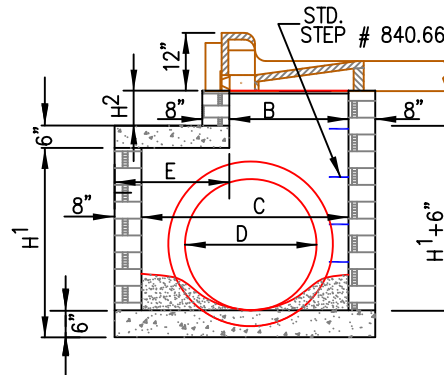
END ELEVATION SECTION J-J
