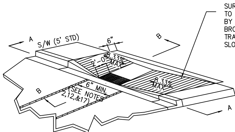
ISOMETRIC VIEW
