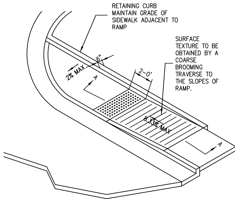
ISOMETRIC VIEW
