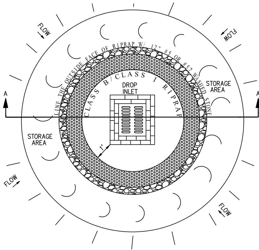
PLAN VIEW
