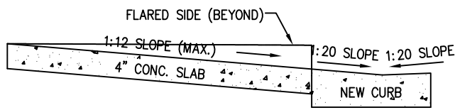
TYP. ROLL CURB SECTION AT HANDICAP RAMP
