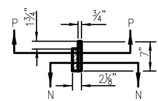
SECTION - MM
