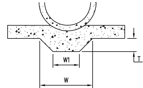
PART SECTION
