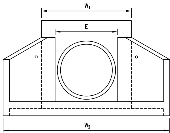
FRONT ELEV.
