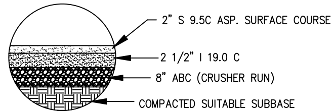
TYPICAL HEAVY COMMERCIAL CROSS SECTION
